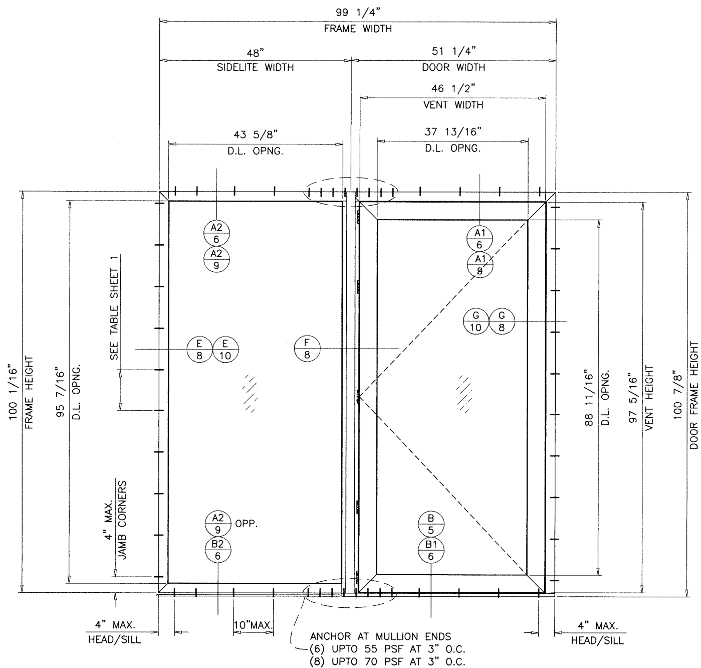
TYPICAL ELEVATION TESTED UNIT
